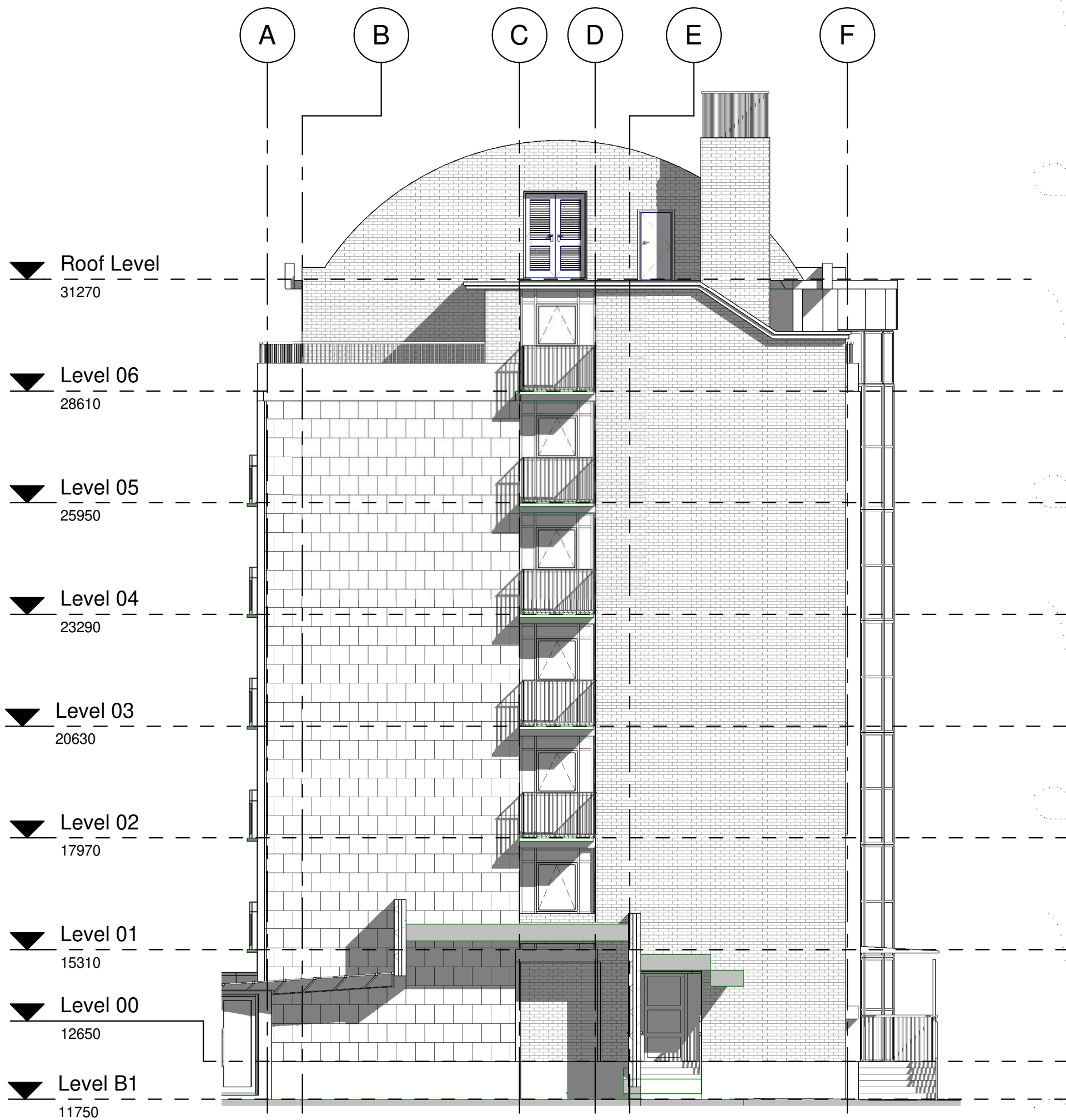
2 Main Building Existing North Elevation 1 : 100
