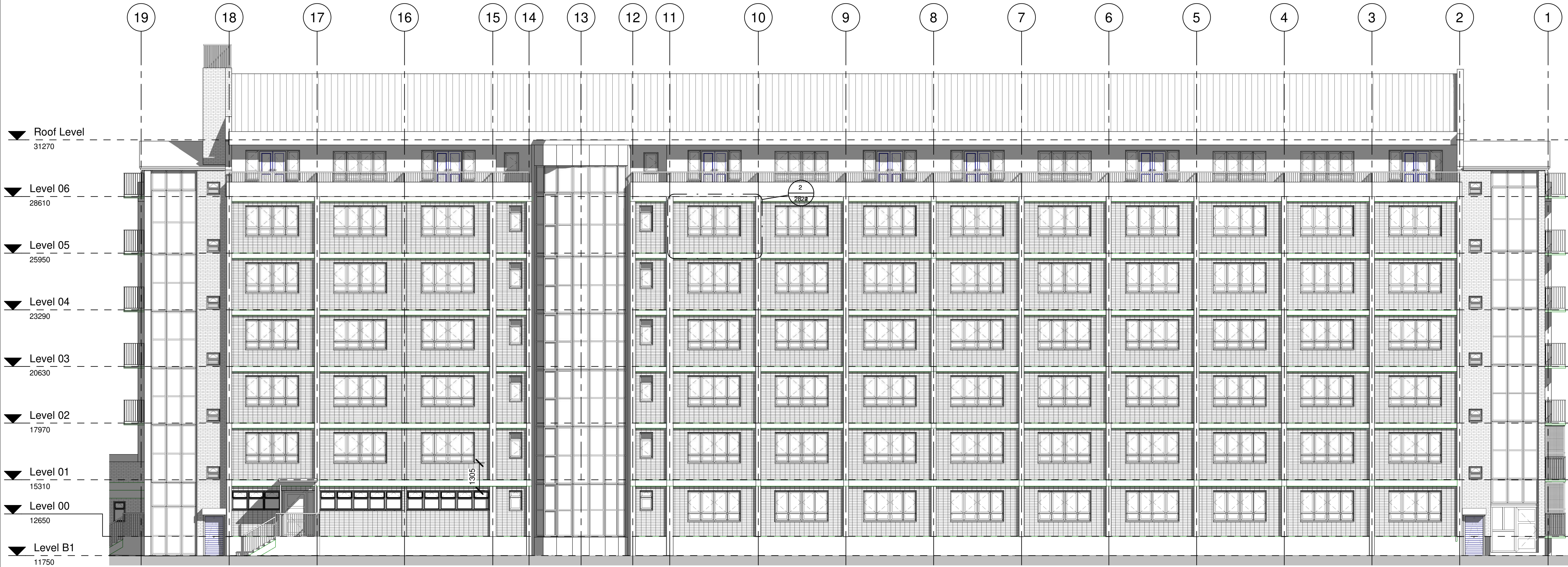
Main Building Existing West Elevation 1 : 100
